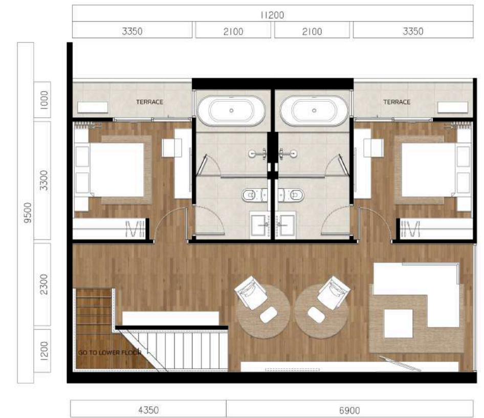
DUPLEX TYPE F ( UPPER FLOOR )
